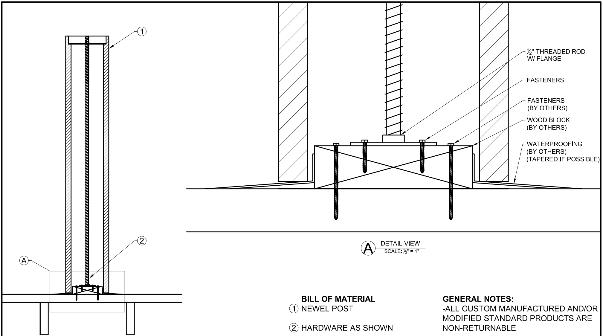
NEWEL INTERNALS SCALE: 3/32" = 1"
