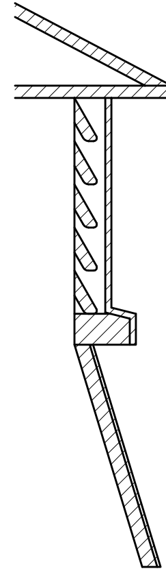
A-A SIDE PROFILE
