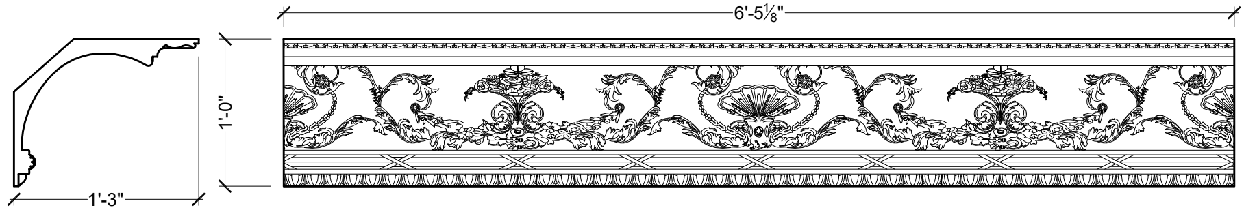
FRONT VIEW
