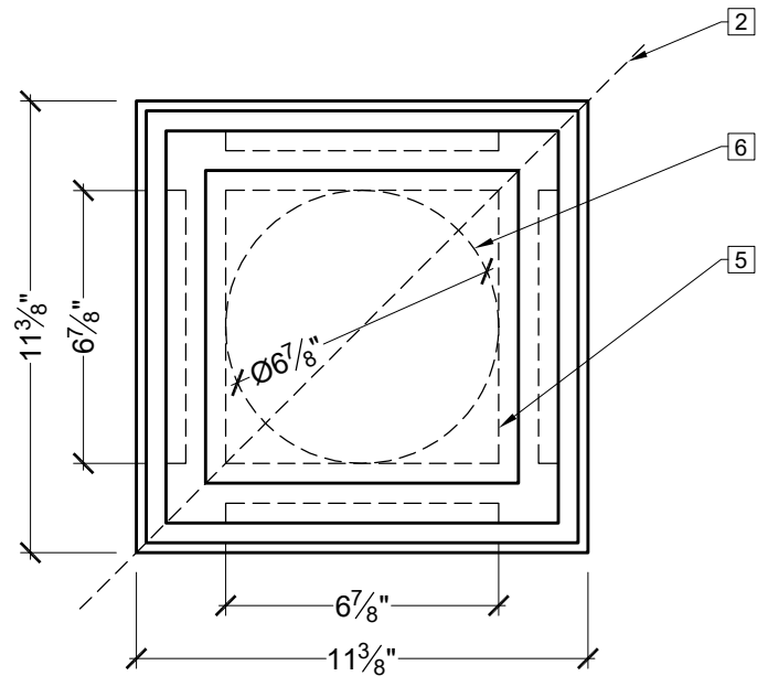
(A) TOP VIEW SCALE: 3/16" = 1"
