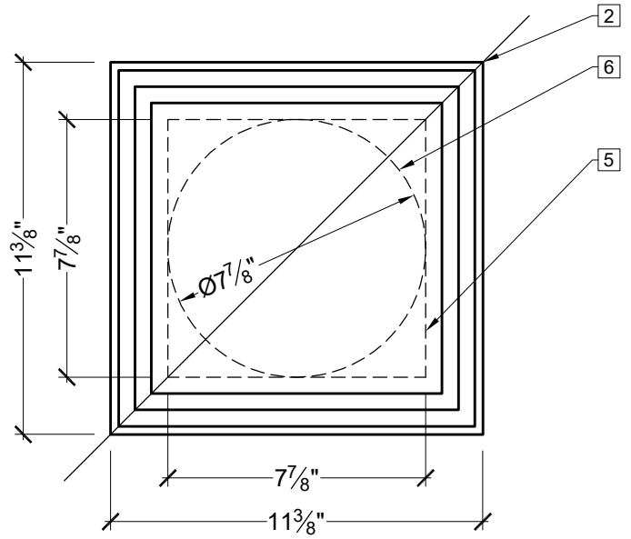
(A) TOP VIEW SCALE: 3/16" = 1"
