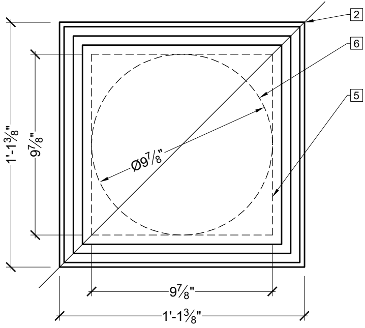
(A) TOP VIEW SCALE: 5/16" = 1"
