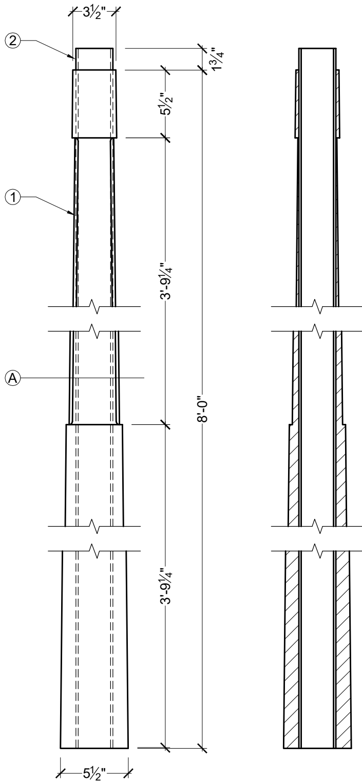
SECTION VIEW
