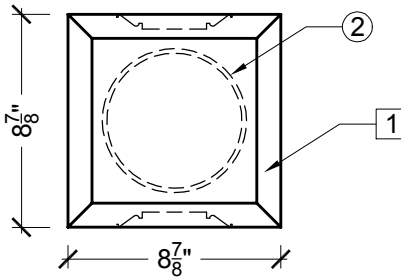
TOP VIEW OF STRAIGHT POST
