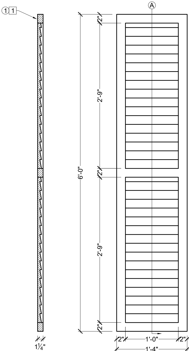
A SECTION VIEW
